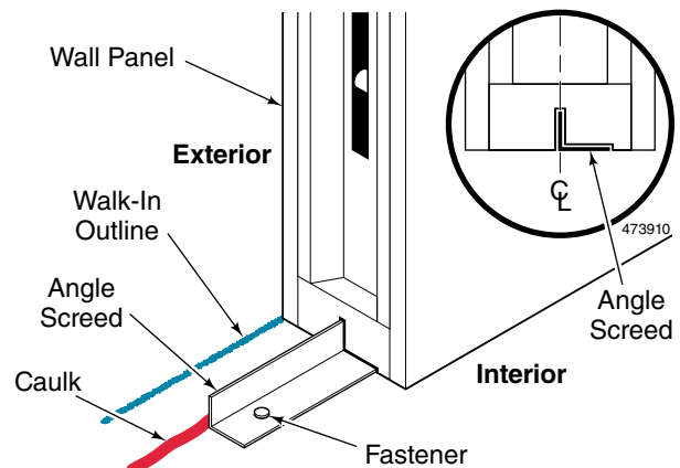
Figure 16. Angle Screed
