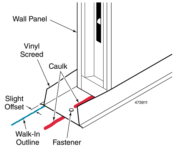
Figure 17. Vinyl Screed
