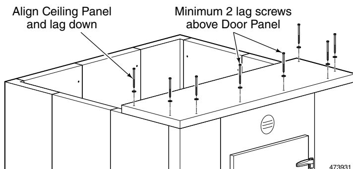
Figure 22. First Panel
