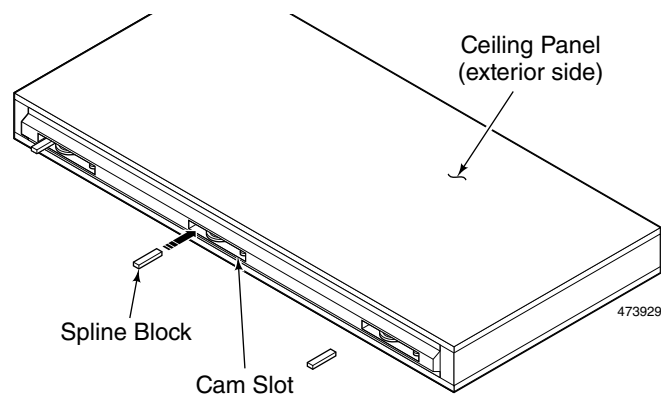
Figure 24. Spline Blocks
