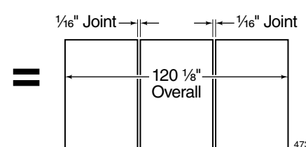
Figure 6. Assembling Panels
