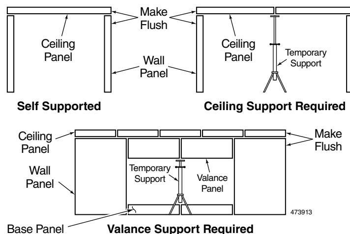
Figure 21. Support
